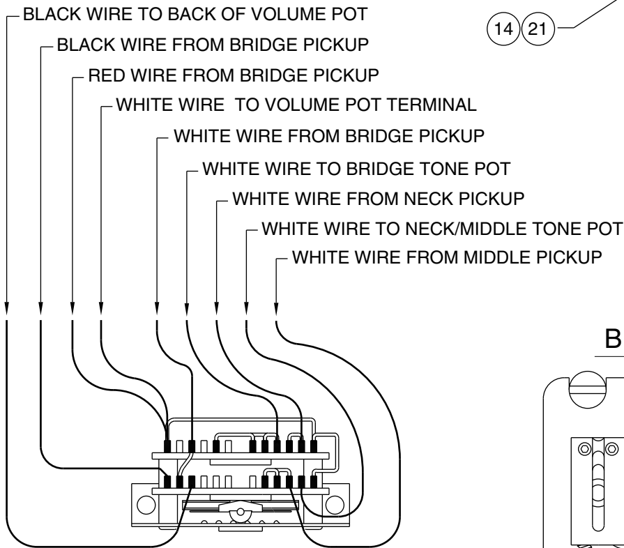
SWITCH WIRING DETAIL
