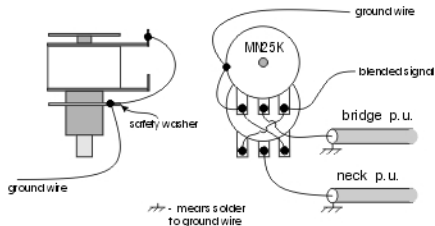
Blend pot wiring viewed from the inside of the control cavity (pot. shaft down)
