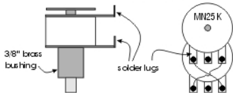
Blend pot wiring viewed from the inside of the control cavity (pot. shaft down)
