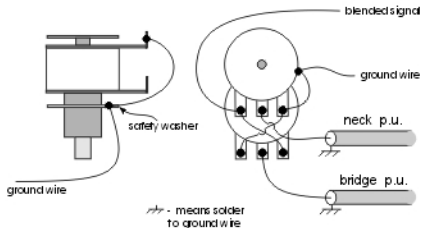
Blend pot wiring viewed from the inside of the control cavity (pot. shaft down)
