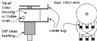
Blend pot wiring viewed from the inside of the control cavity (pot. shaft down)
