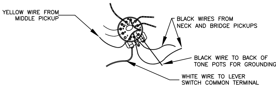
S-1 SWITCH WIRING DETAIL
