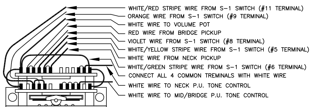
LEVER SWITCH WIRING DETAIL
